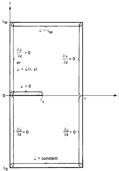
FIG. 2. Boundary condition used on \chi, \lambda grid for 2-D calculation.
