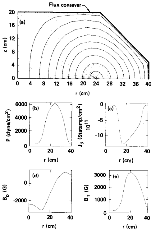
FIG. 3. CTX equilibrium, (a) \chi, \lambda grid, (b) pressure vs. r at z = 0 , (c) toroidal current vs. r at z = 0 , (d) poloidal magnetic field vs. r at z = 0 , (e) toroidal magnetic field vs. r at z = 0 .
