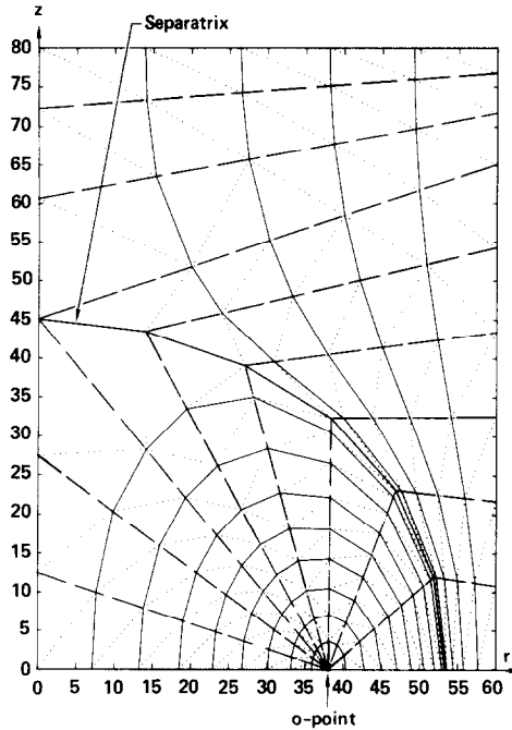
FIG. 1. \chi, \lambda grid. Dark lines are surfaces of constant \chi . Dashed lines are surfaces of constant \lambda . Dotted lines denote boundary of finite elements.
