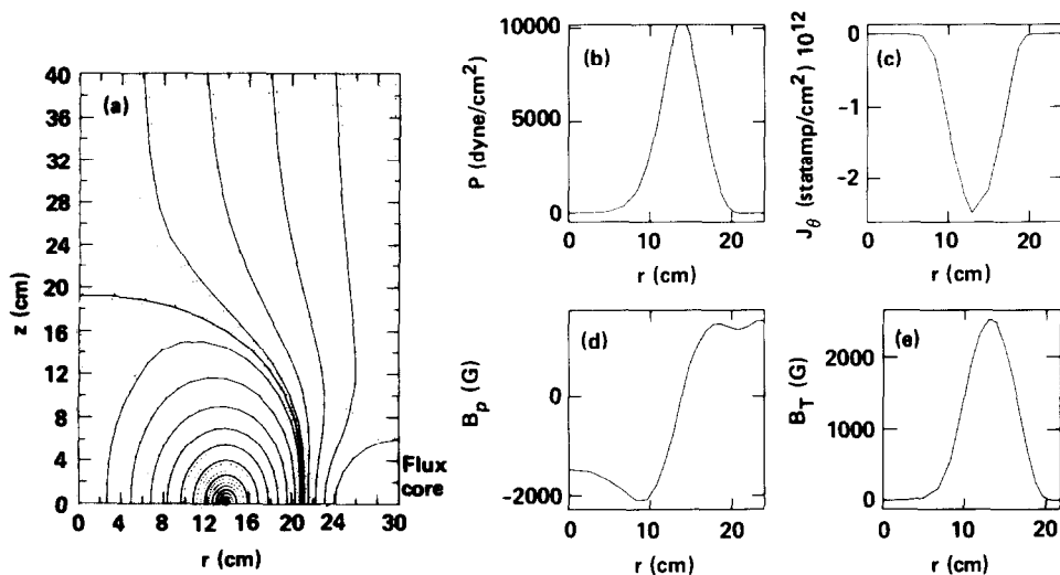
FIG. 4. Proto S-1C equilibrium, (a) \chi, \lambda grid, (b) pressure vs. r at z=0 , (c) toroidal current vs. r at z=0 , (d) poloidal magnetic field vs. r at z=0 , (e) toroidal magnetic field vs. r at z=0 .
