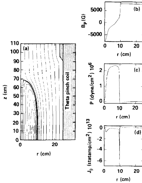
FIG. 5. FRC equilibrium, (a) \chi surfaces, (b) poloidal magnetic field vs. r at z=0 , (c) pressure vs. r at z=0 , (d) toroidal current vs. r at z=0 .
